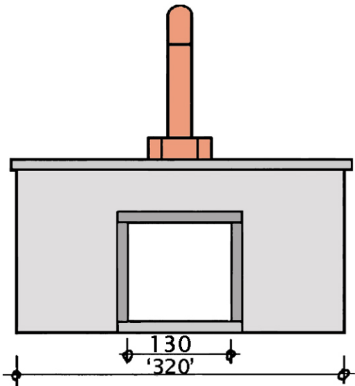
SIDE ELEVATION showing end of tunnel
